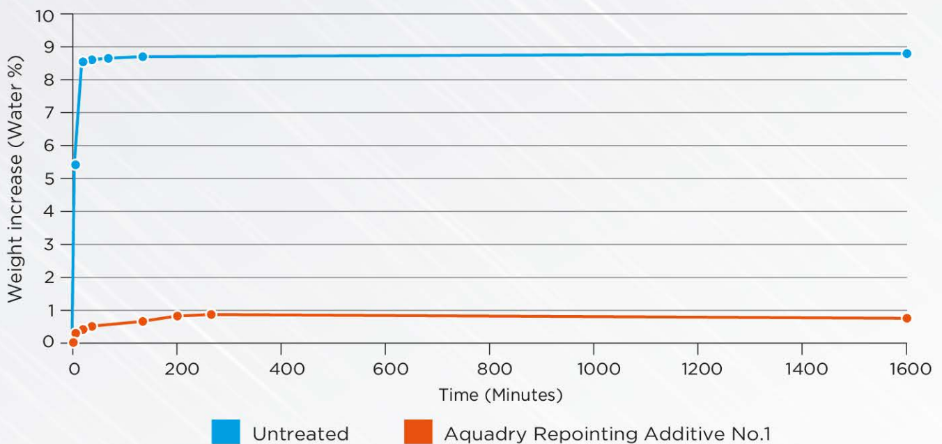
The reduction in water absorption of repointing masonry after the addition of Aquadry Repointing Additive No. 1
